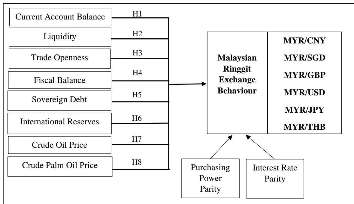
Figure 2: Research Framework
